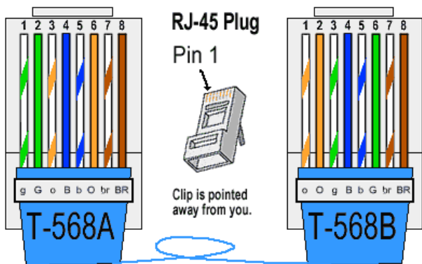
Color Standard EIA/TIA T568A
