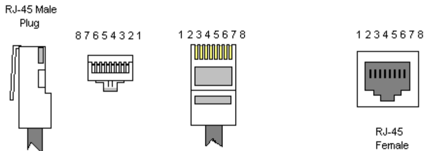
Color Standard EIA/TIA T568A
